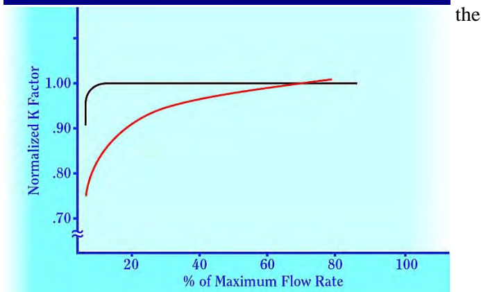
Figure 4 • Viscosity Effects on 1" Flow-
